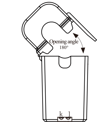
Output screw terminal
