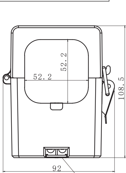
Front view Output screw terminal
